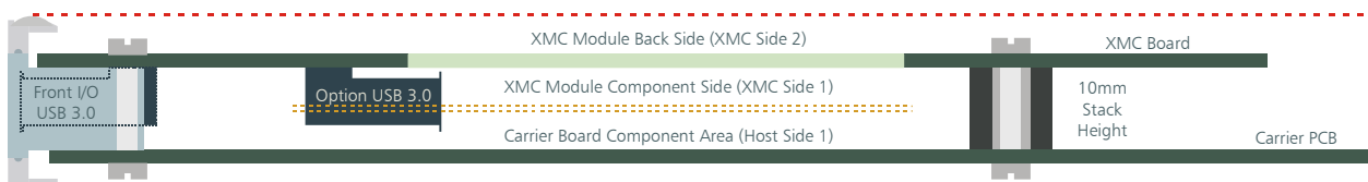
DB4-EAGLE on a CPCI Carrier Board - Sectional Drawing • © EKF • ekf.com
